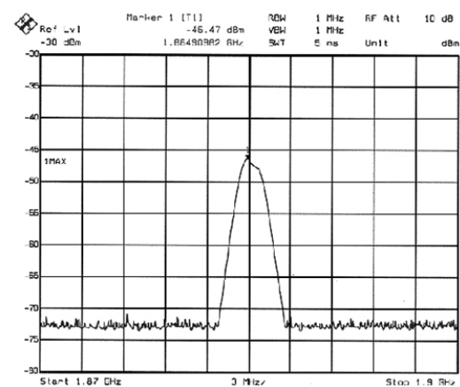
Fig. 1. Analysis of frequency for the active DECT base (Siemens Gigaset 4010 Classic) ranging from 1.87 GHz to 1.90 GHz
